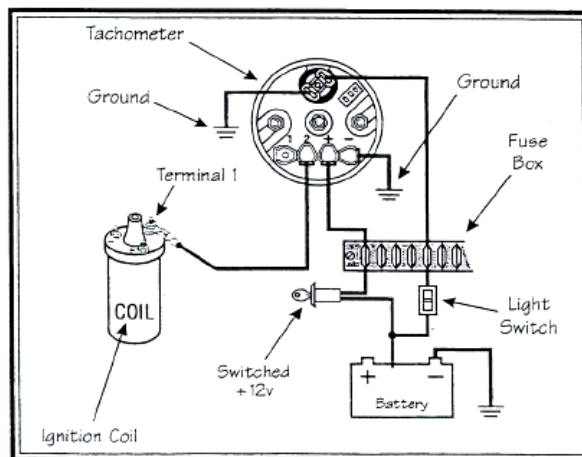
Diagram D Proper wiring of the VDO Tachometer with the Ignition Coil
