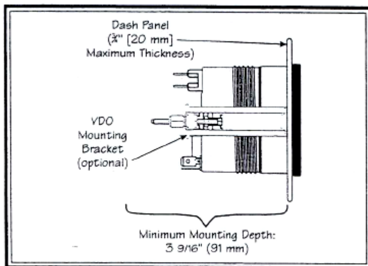
Diagram C Mounting with the optional VDO Mounting Bracket
